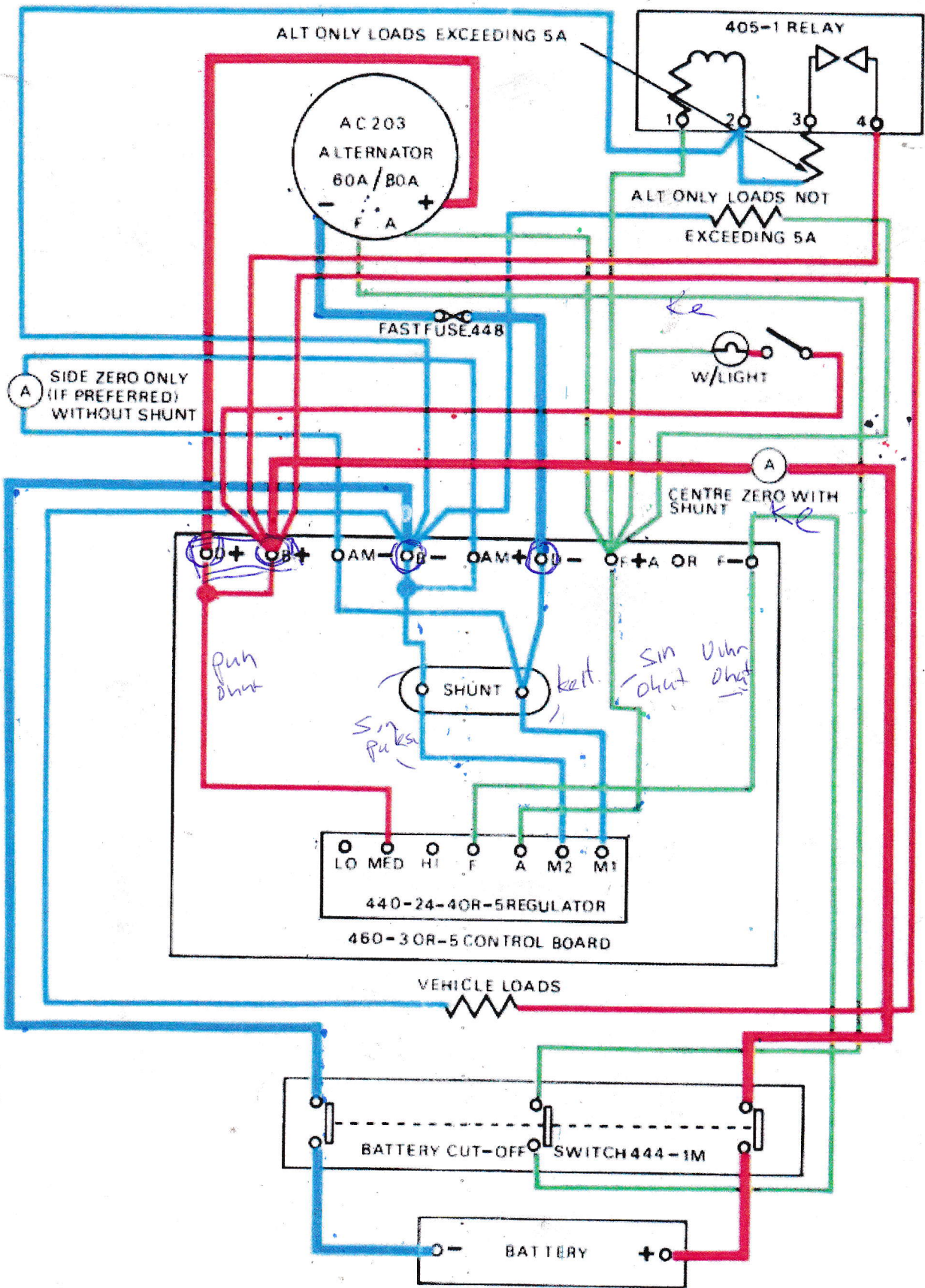
Fig 20 Typical AC203 system
